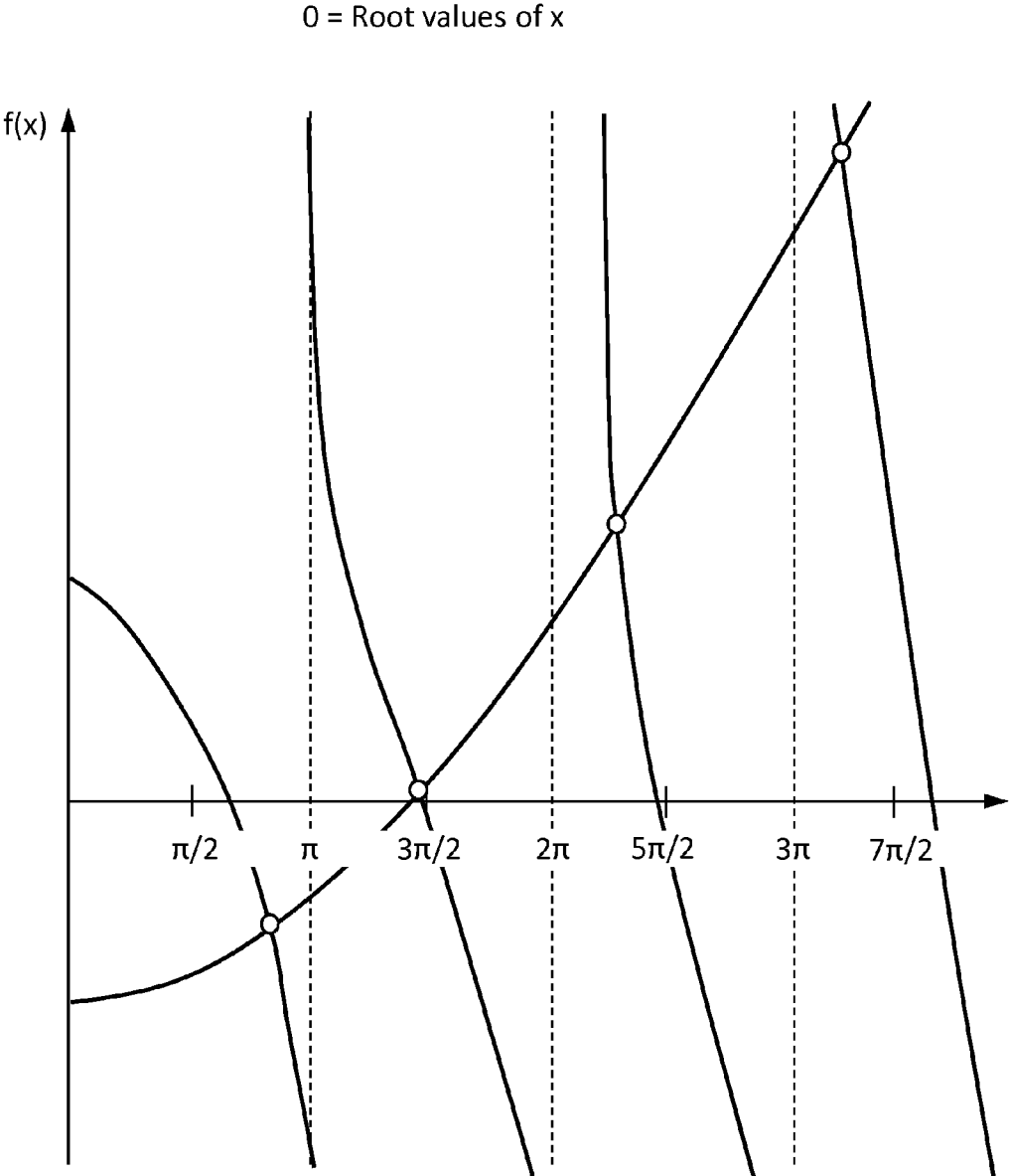
Graphical determination of pole locations
