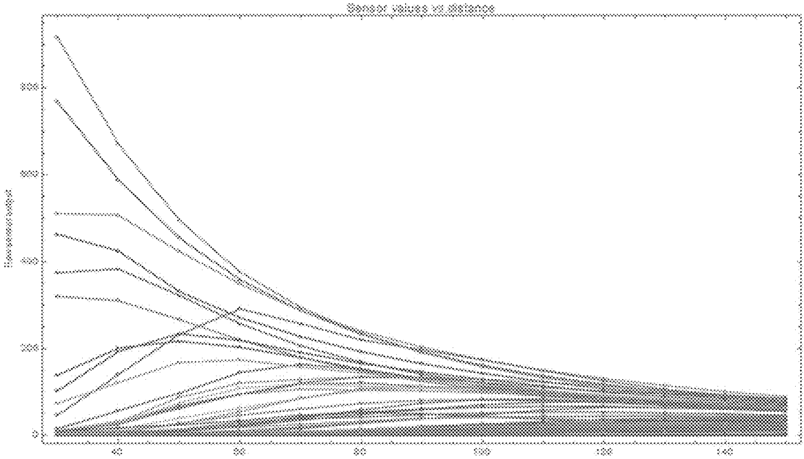
Piecewise-Linear Interpolation Between Measured-Dataset Separation-Distances
